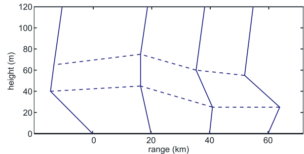
Figure 9. Example of range-dependent 16-parameter M profile with 4 parameters per 20 km. Vertical profile at any given range is calculated by linear interpolation of both the slopes and the layer thicknesses.
